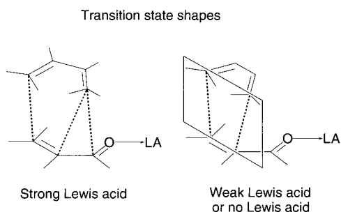
Fig. 8.7 The different transition-state shapes for the carbo-Diels-Alder reaction in the presence of a strong Lewis acid (left) – a three center interaction – and a weak Lewis acid (right) [12]
