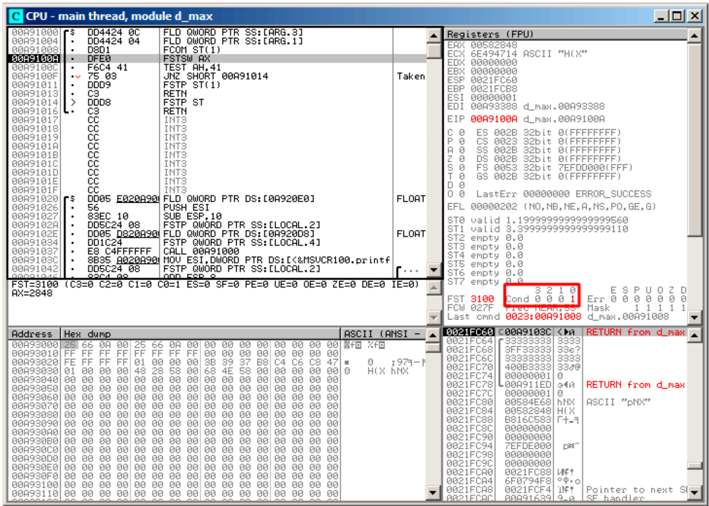
Figure 1.79: OllyDbg: FCOM has been executed
