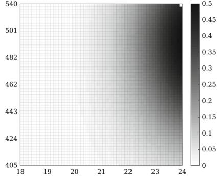
Fig. 1. Case study 1: Lower bound probability of satisfying \varphi_1 generated using IMDP with 3481 states.
