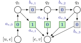
(a) PERT network \mathbf{PN} . (b) Gadget for e = (u, v) with rational weights p_e, \bar{p}_e . (c) Equivalent gadget for e with weights 1 for p_e = 5/8 = (0.101)_2 .
