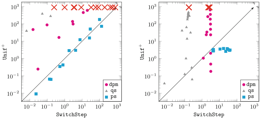
Fig. 4. Running times of algorithms SwitchStep and Unif + .
