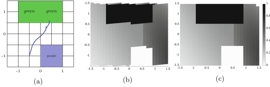
Fig. 2. Case study 2: (a) Gridded domain together with a superimposed simulation of trajectory initialised at (-0.5, -1) within q_0 , under the synthesised optimal switching strategy \pi^* . Lower probabilities of satisfying \varphi_2 for mode q_0 (b) and for mode q_1 (c), as computed by StochHy .
