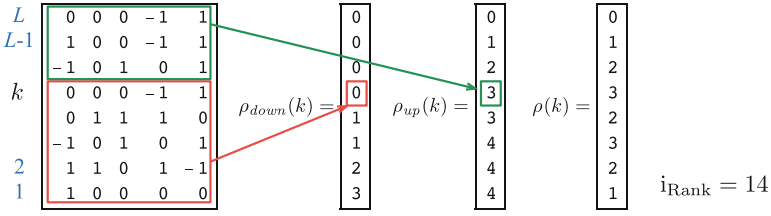
Fig. 4. Computations of the rank weights from a matrix \mathbf{F} with \text{rank}(\mathbf{F}) = 4 .
