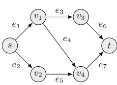
(a) PERT network \mathbf{PN} . (b) Gadget for e = (u, v) with rational weights p_e, \bar{p}_e . (c) Equivalent gadget for e with weights 1 for p_e = 5/8 = (0.101)_2 .
