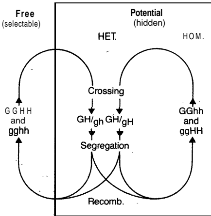
Fig. 21b. The states of variability in a system where the G and H loci are additive in effect on phenotype, so that GgHh and GGhh are phenotypically identical. The extremes of phenotype (free variability) are expressed by the double dominant and double recessive .
