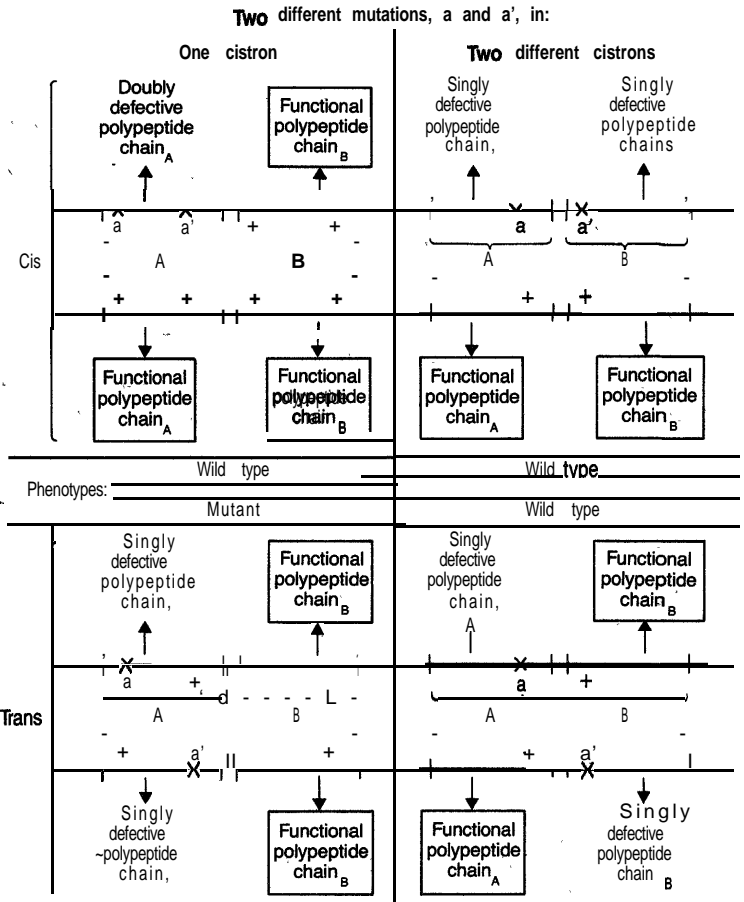
Fig. 10. Theoretical basis of the cis-trans test. Where two mutations (—x—) occur within the same chromosome ( cis configuration), complementation occurs through functional polypeptide production by the complementary cistron or cistrons of the other chromosome. Mutant phenotype only occurs where the two mutations occur within the same cistron but on different chromosomes. This effect enables precise mapping of the physical limits of cistrons within chromosomes.
