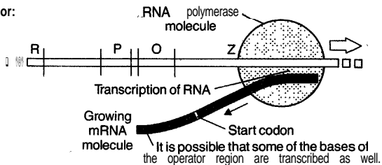
Fig. 39. Simplified diagram indicating the effect of a repressor molecule (a&owe) in inhibiting transcription of gene Z by RN A polymerase compared with loss of this inhibition (below) when it is removed. Gene t? encodes the repressor. © J. D. Watson: Molecular Biology of the Gene 3rd ed. (1976), Fig 14-12(a). Pub. Benjamin/Cummings.
