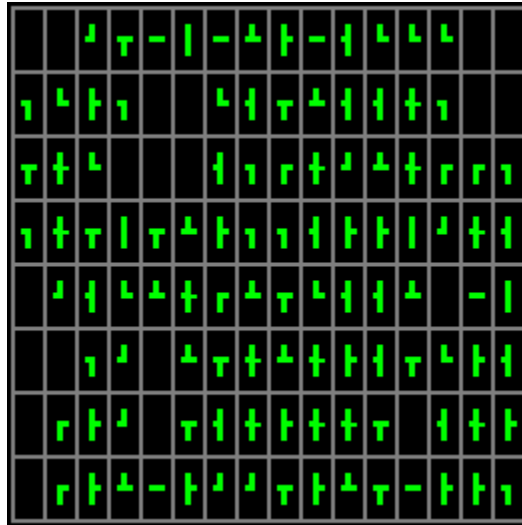
Figure 8.3: Shuffled puzzle
