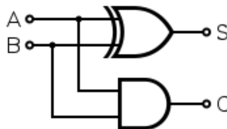
Figure 3.5: Half-adder
