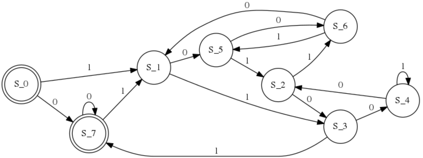
Figure 15.11: DFA for numbers divisible by 7
