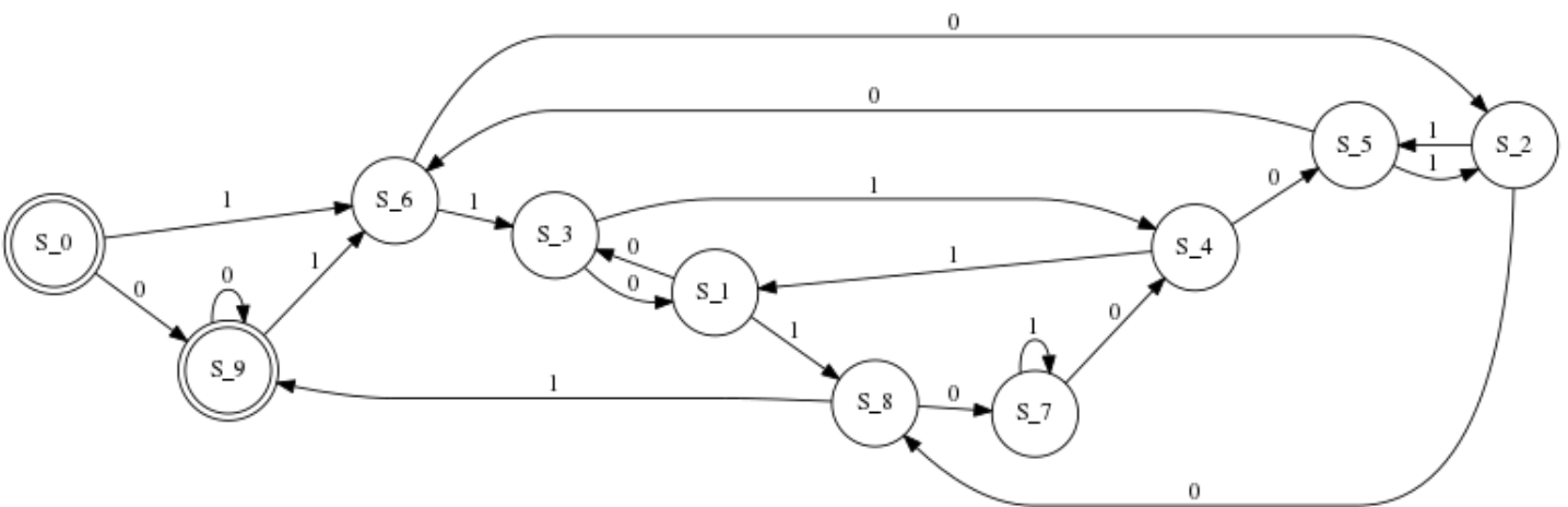
Figure 15.12: DFA for numbers divisible by 9. Probably not an easy thing to find it manually
