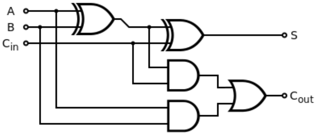
Figure 3.6: Full-adder
