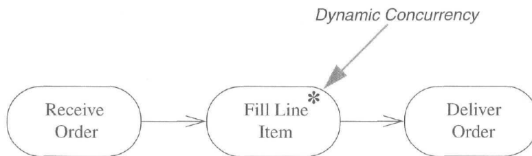
Figure 9-4: Dynamic Concurrency
