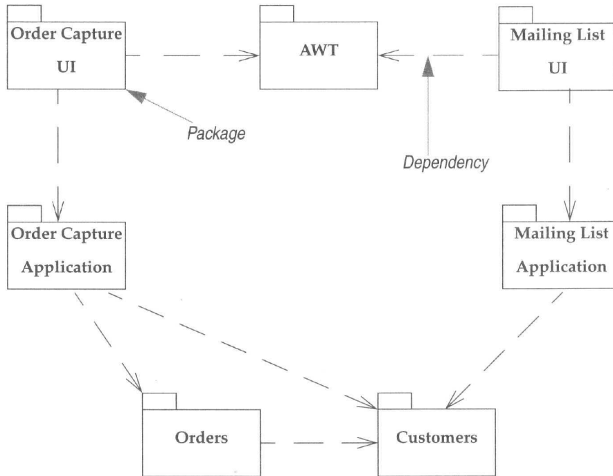
Figure 7-1: Package Diagram
