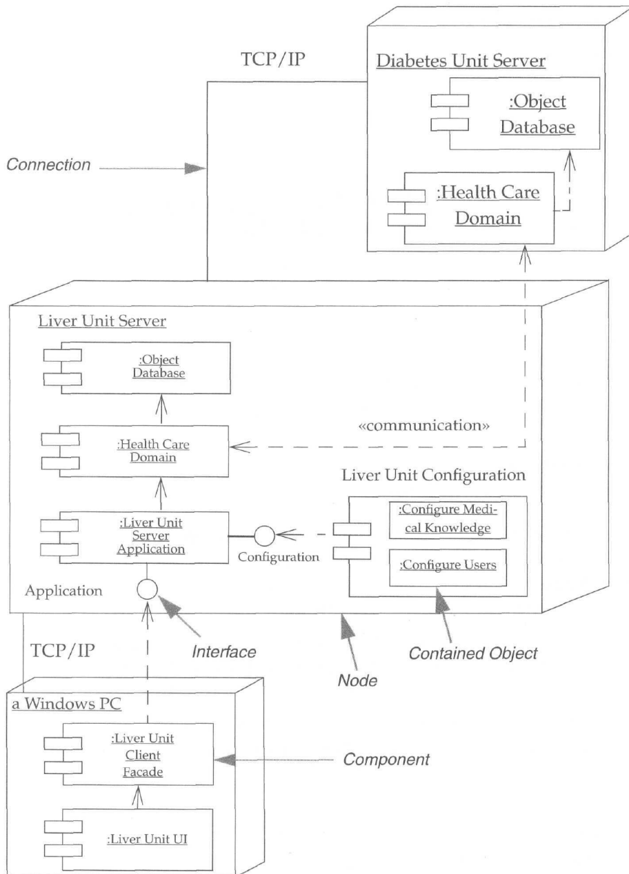
Figure 10-1: Deployment Diagram
