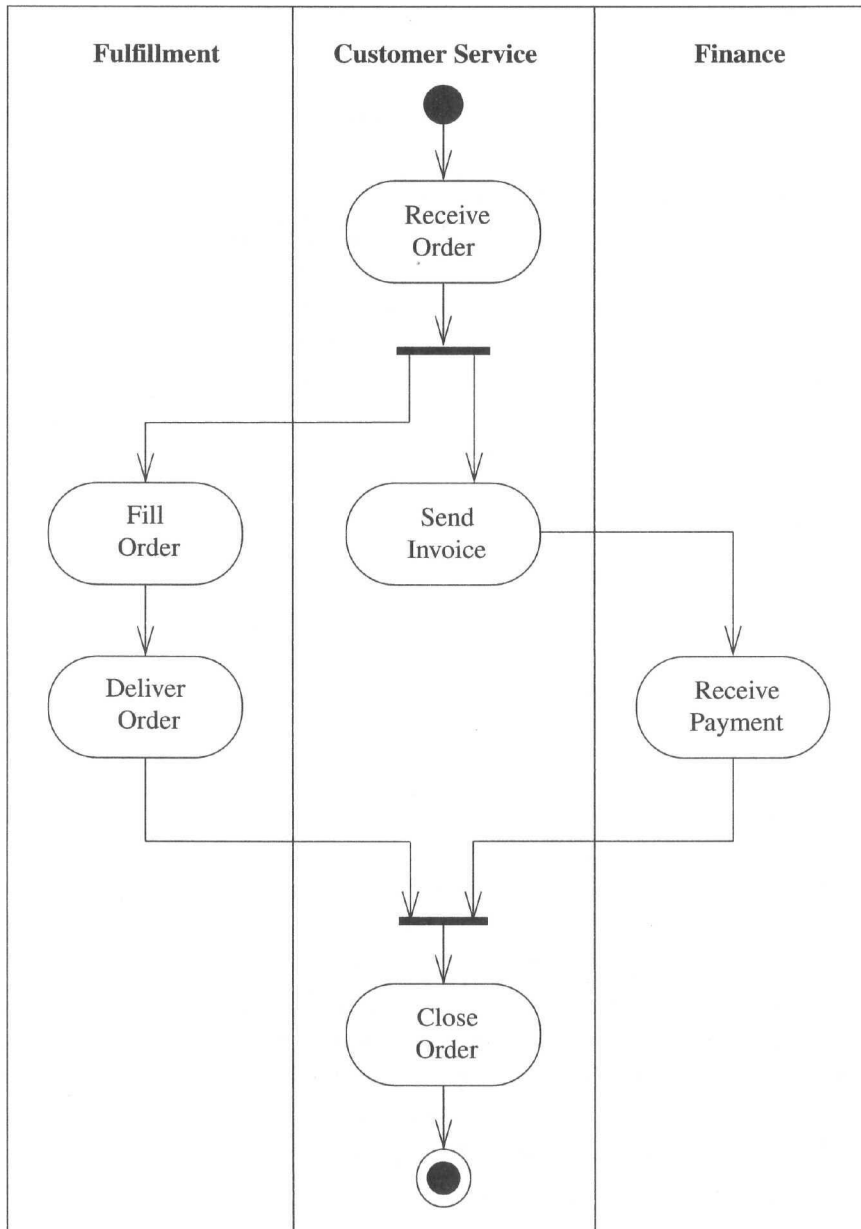
Figure 9-5: Swimlanes
