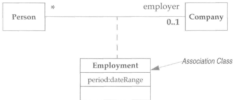
Figure 6-14: Association Class
