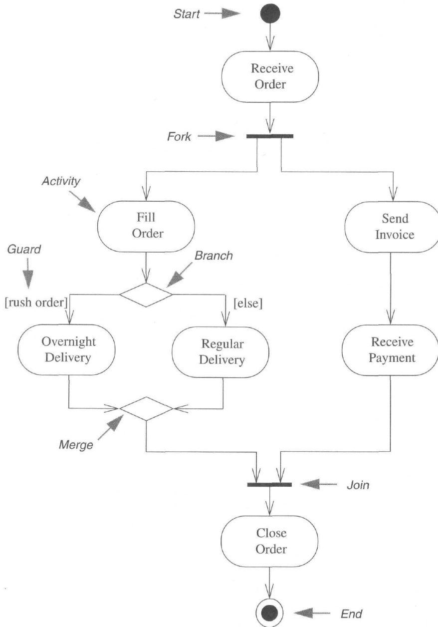
Figure 9-1: Activity Diagram
