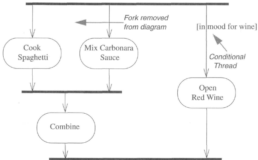
Figure 9-2: Forks, Joins, and Conditional Threads
